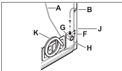
Braided flexible stainless steel tubing installation
