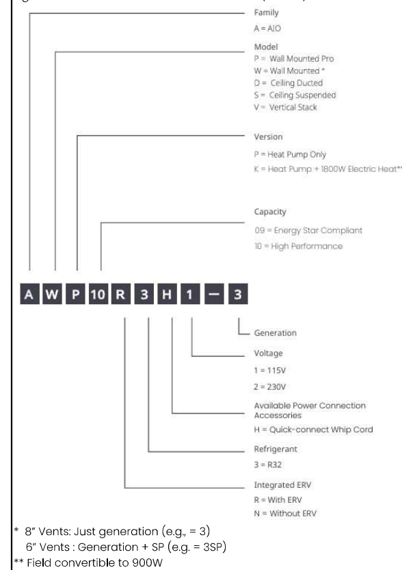
Figure 1. AIO Wall Mounted Standard & Pro (Gen 2/3) nomenclature
